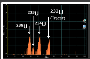
alpha-ray spectrum of Uranium isotopes
