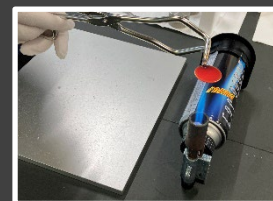
Red-heating after electrodeposition
