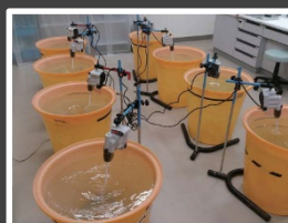
Seawater pretreatment
